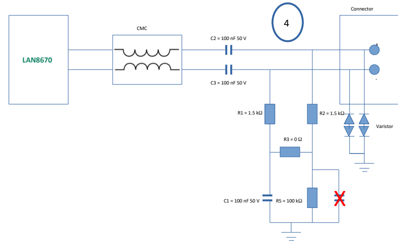
Drop Node Termination
