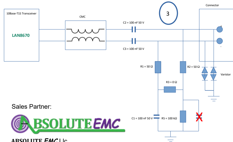
End Node Termination
