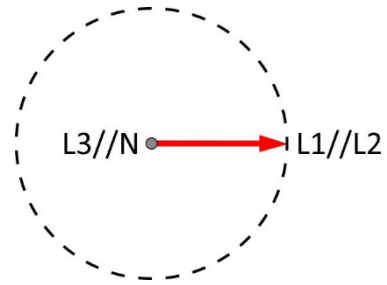
Figure 10: Phase Connection '1L (AC/DC double current)'
