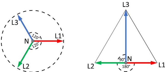
Figure 9: Phase Connection '3L (AC/DC)'
