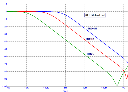
S21 on a 1 M \Omega load
