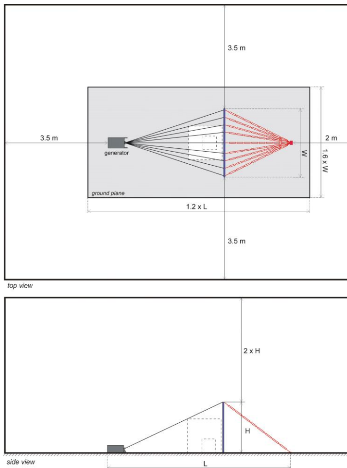
Fig. 11: minimum recommended clearance distances (for small NEMP test installations)
