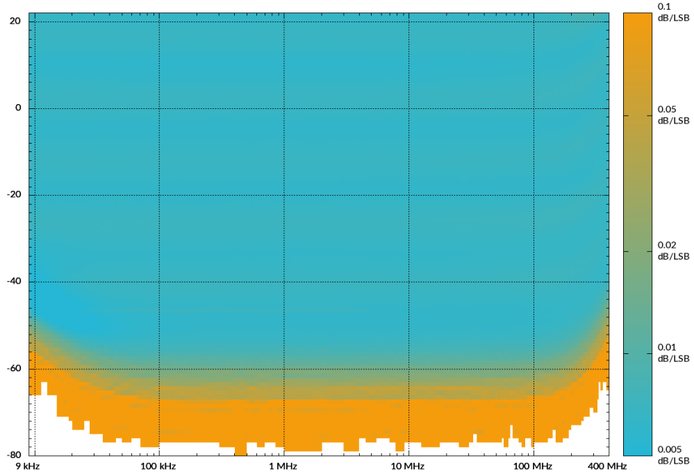
Figure 48: Typical dynamic range, low band
