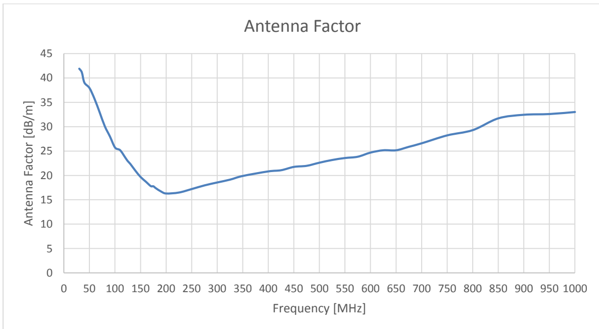
30 MHz...1 GHz , Antenna Factor of TBMA1
