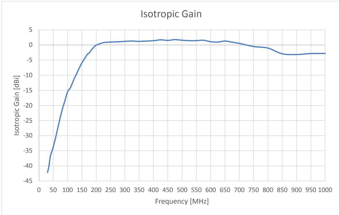
30 MHz...1 GHz , Isotropic Gain of TBMA1
