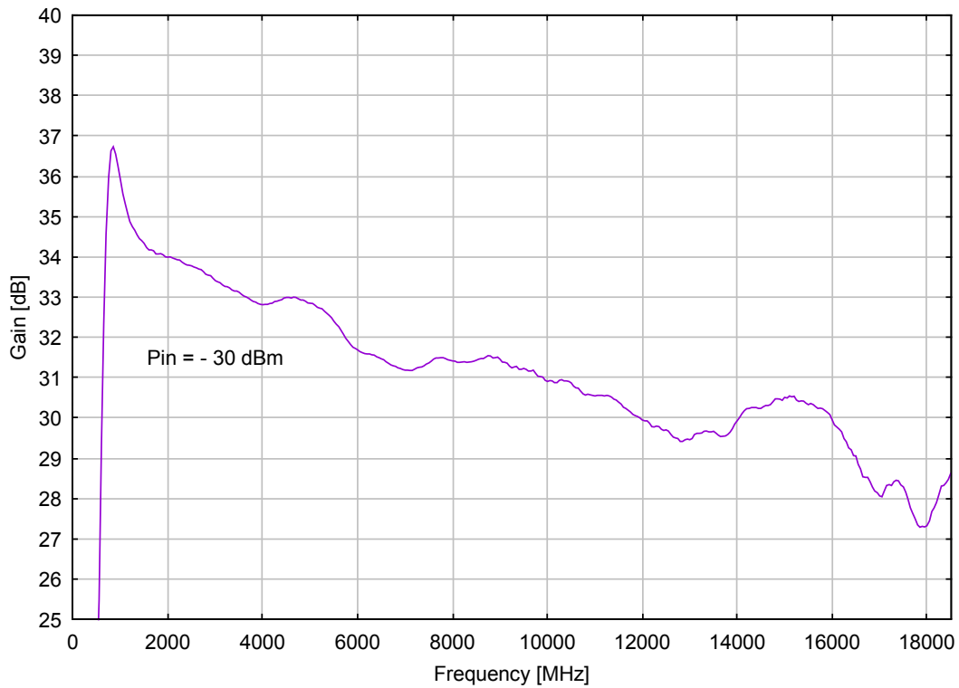
BBV 9718 C + 0.5 m Cable N/SMA
