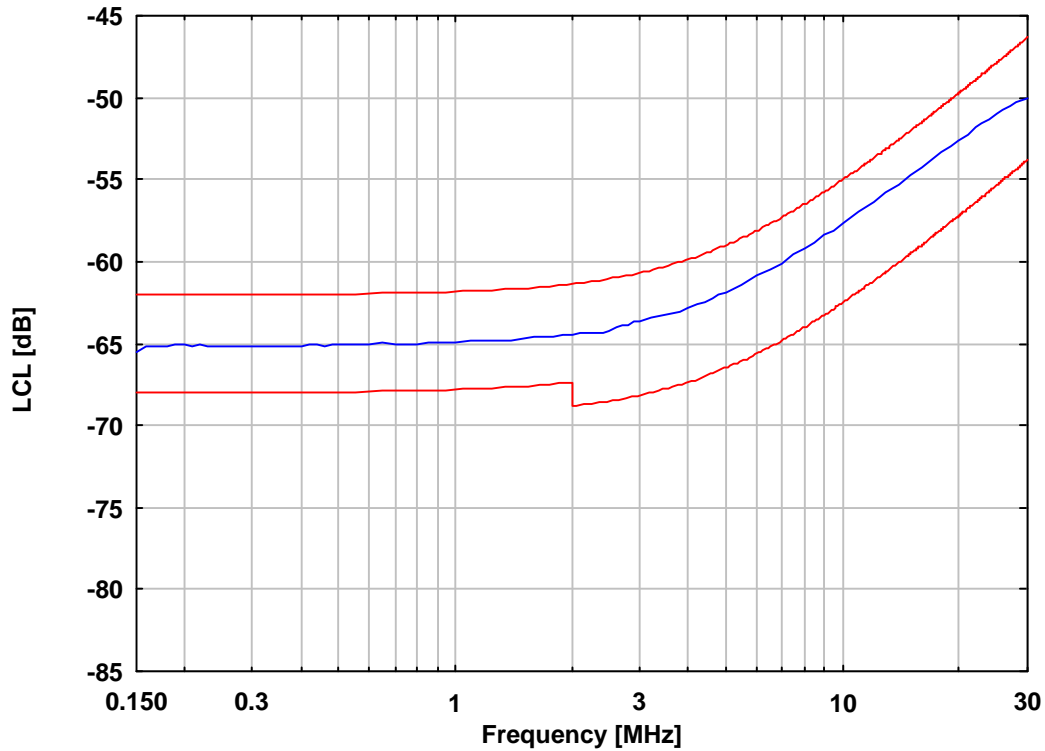
Longitudinal Conversion Loss (LCL)
