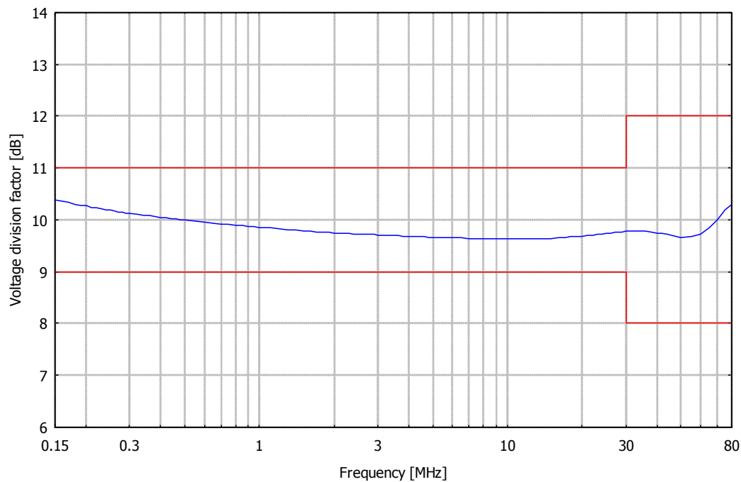
Transmission EuT to Measurement Port
