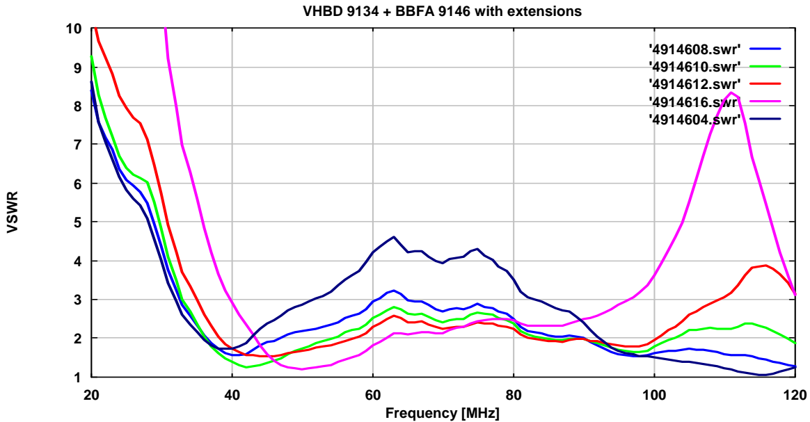
VHBD 9134 with BBFA 9146 with Extensions opened to diameters of 0.4 m to 1.6 m measured at the element junction.
