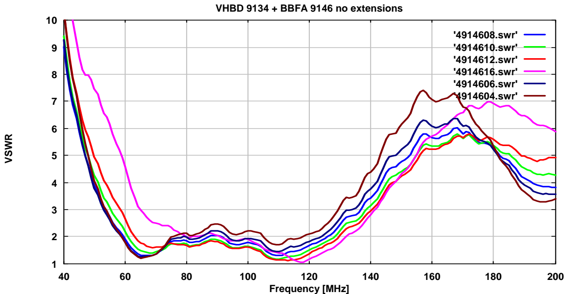
VHBD 9134 with BBFA 9146 without Extensions opened to diameters of 0.4 m to 1.6 m measured at the element junction.
