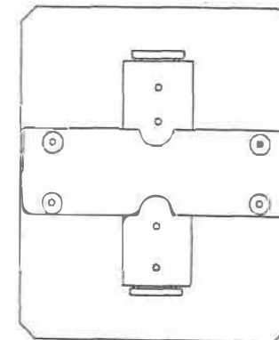
UHAP Calibration Adapter
