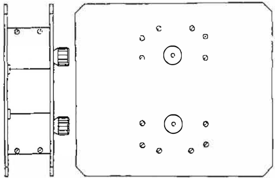
VHAP CALIBRATION ADAPTER 30 – 300 MHz
