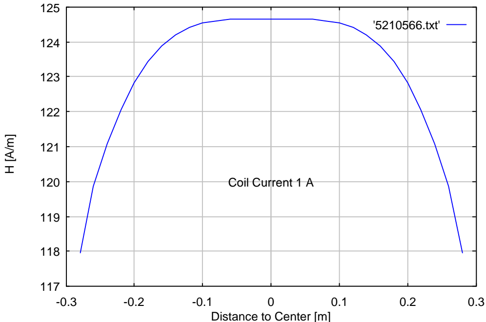
Spulenabstand 0.566 m Coil Distance 0.566 m HHS 5210-100 magnetic fieldstrength along longitudinal coil axis
