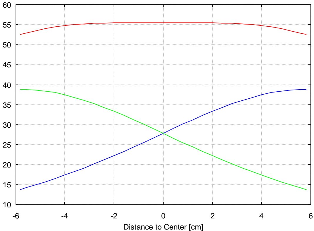
HHS 5202-9 magnetic Fieldstrength along longitudinal coil axis
