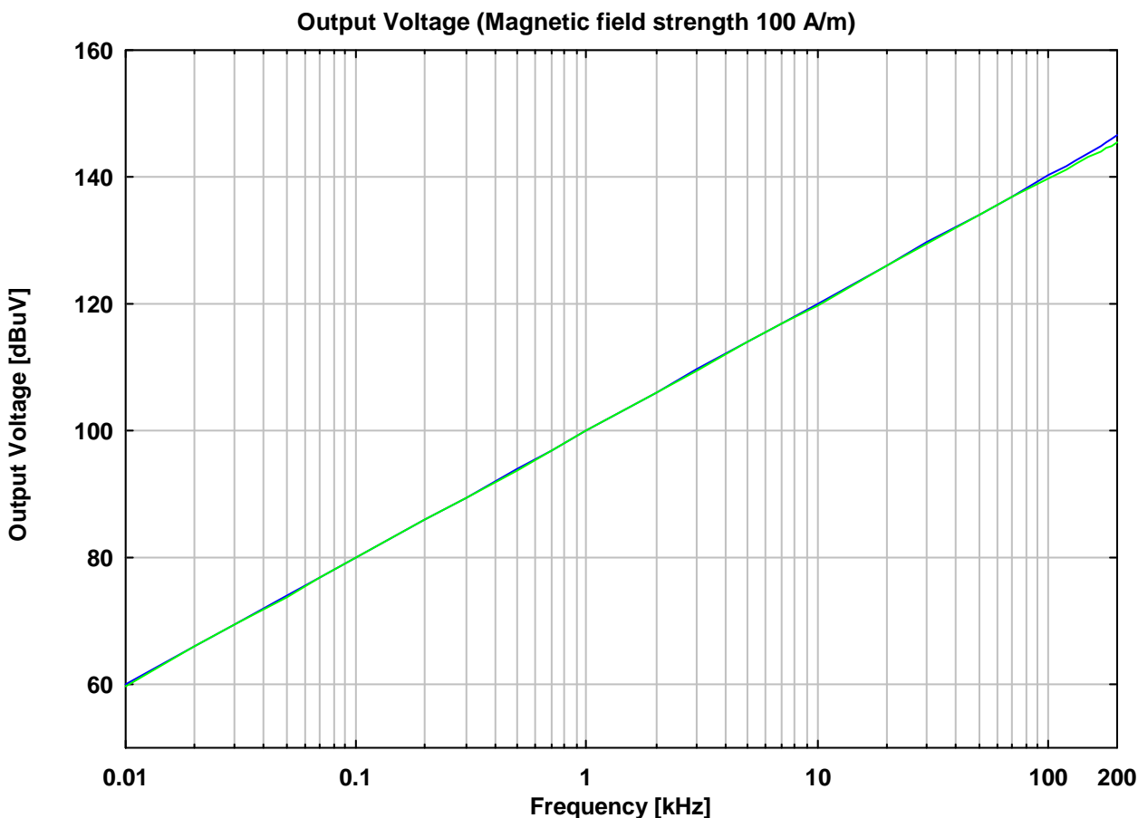
Blue Line: Open circuit voltage, Green Line: Voltage across 50 Ω load.
