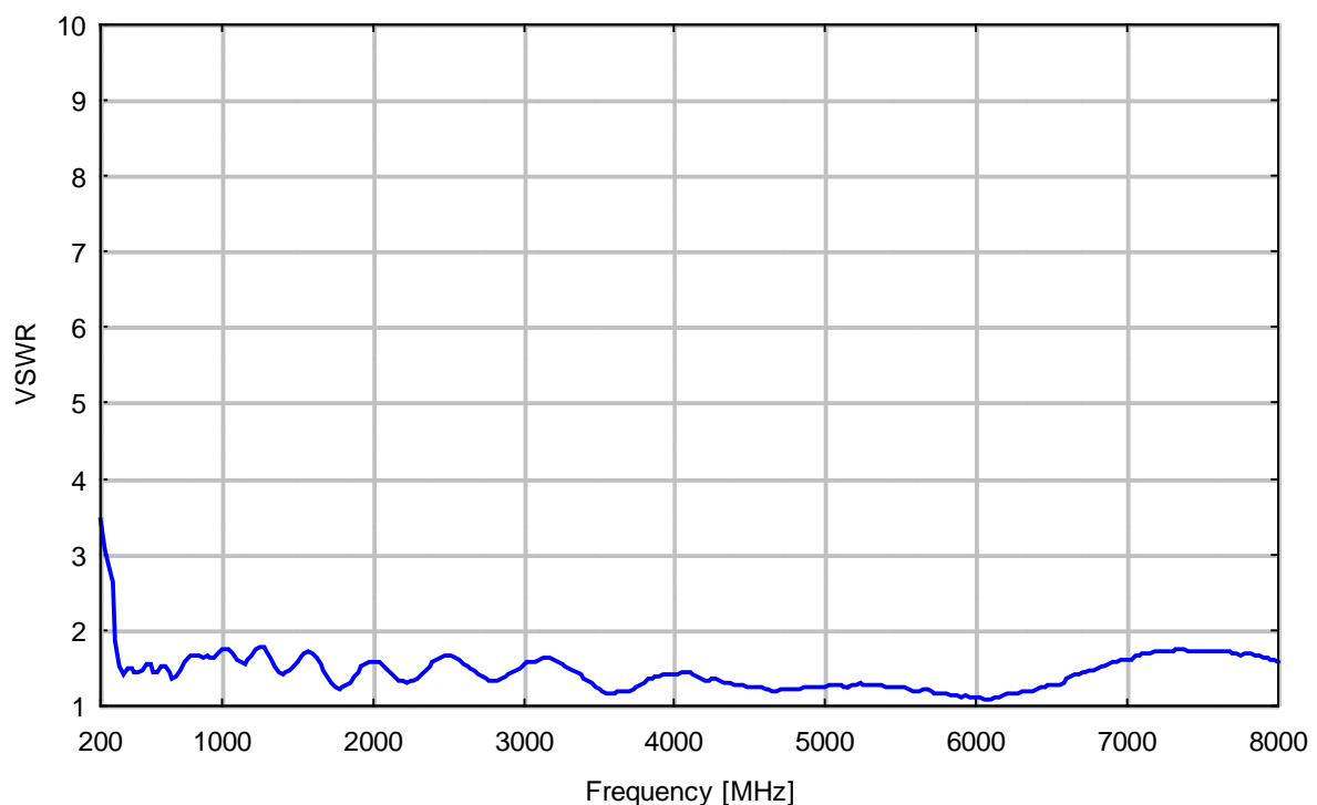
USLP 9143 Individual VSWR
