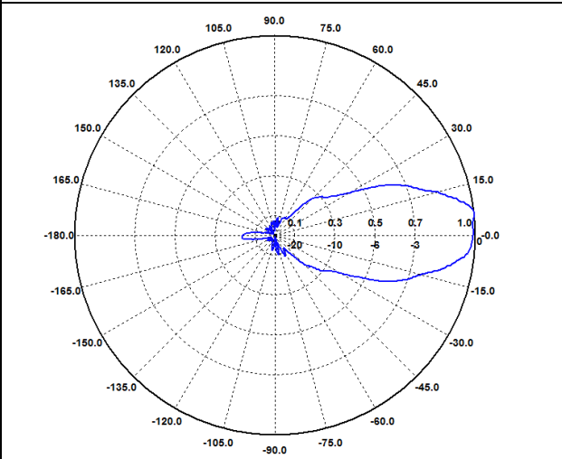
H-Ebene / H-Plane 1600 MHz
