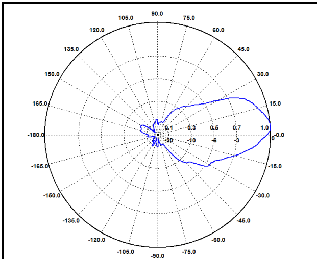
E-Ebene / E-Plane 1400 MHz
