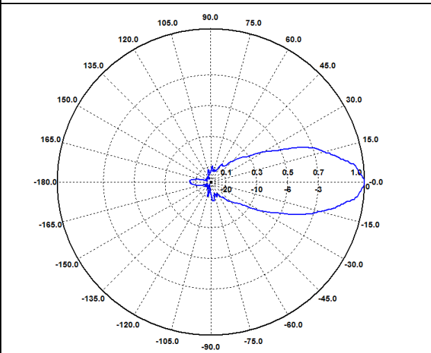
H-Ebene / H-Plane 1800 MHz
