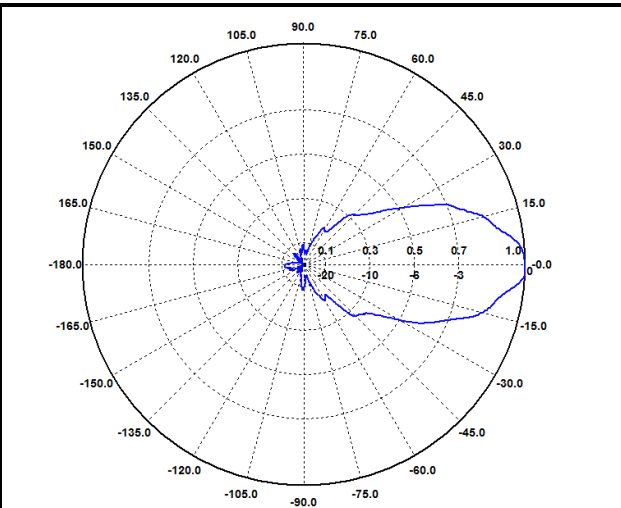
H-Ebene / H-Plane 1400 MHz
