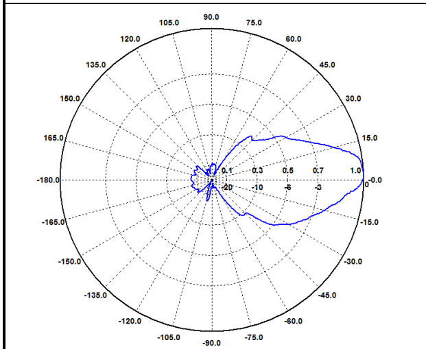
E-Ebene / E-Plane 1800 MHz
