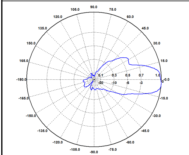
E-Ebene / E-Plane 1600 MHz
