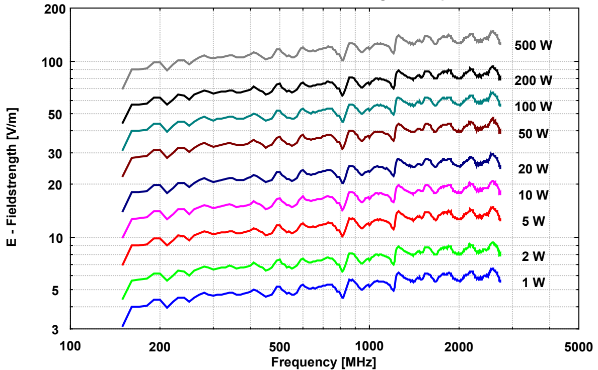
STLP 9128 C Generated Fieldstrength 3 m Tip - EuT
