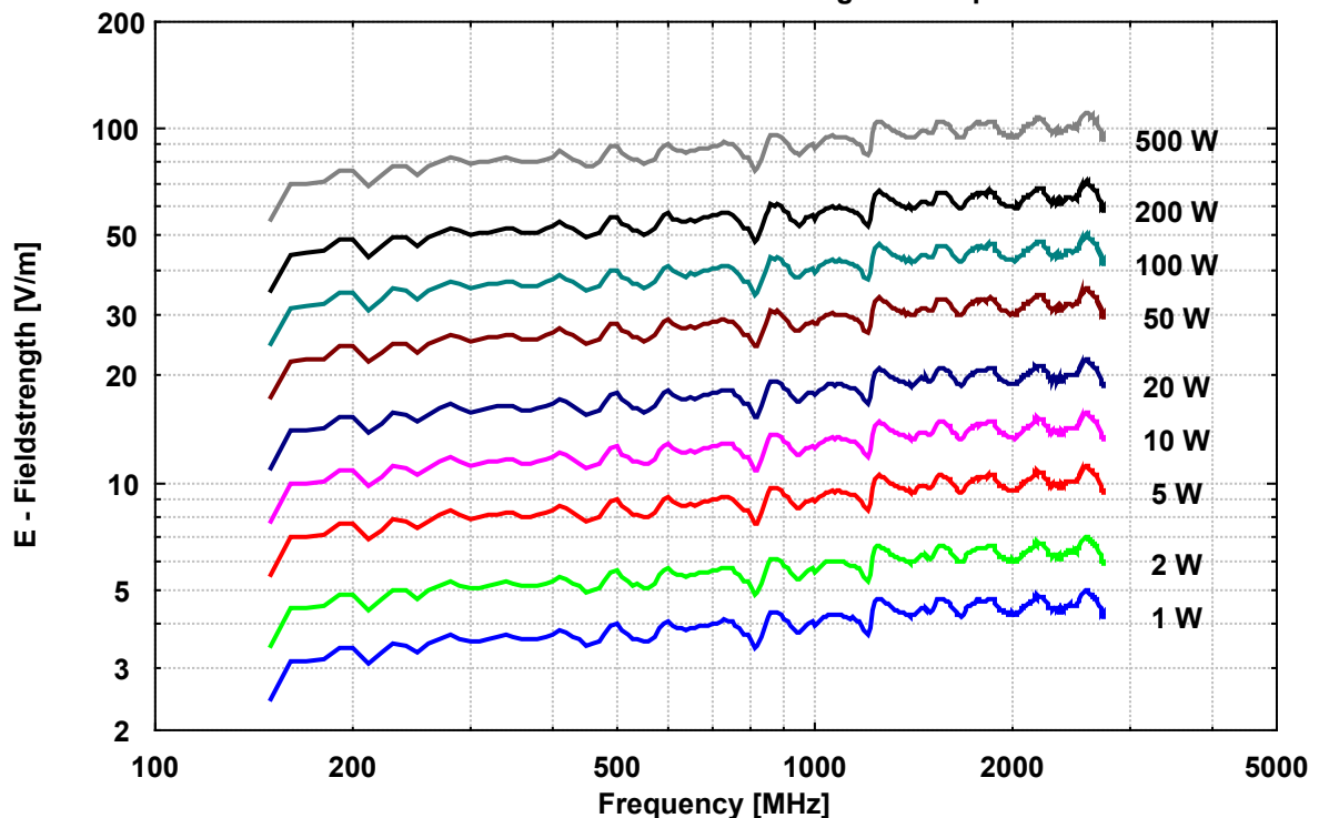
STLP 9128 C Generated Fieldstrength 4 m Tip - EuT
