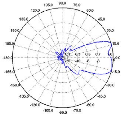
E-Ebene / E-Plane 1.2 GHz
