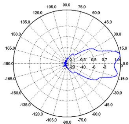
E-Ebene / E-Plane 1.6 GHz
