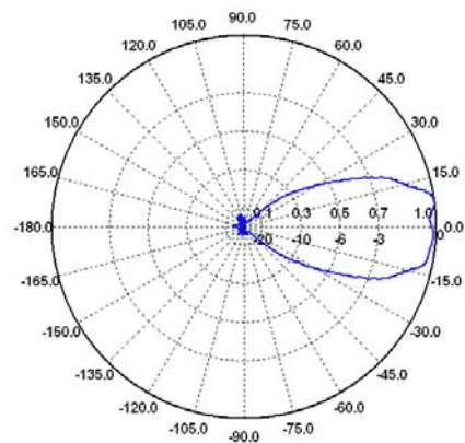
H-Ebene / H-Plane 1.6 GHz
