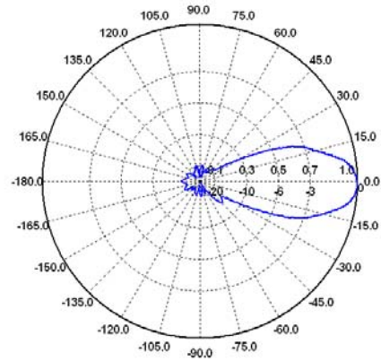
H-Ebene / H-Plane 1.2 GHz
