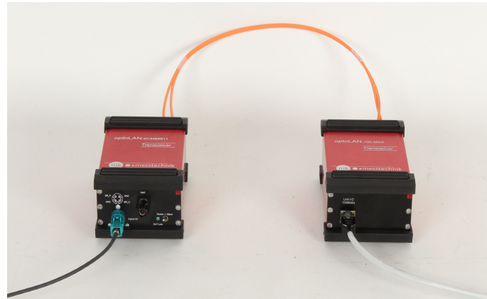
BroadR-Reach optical link T1 to Tx
