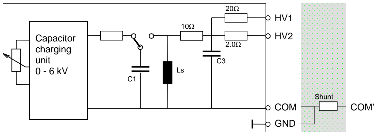
Figure 1: Ring-Wave Generator IPG 612T, schematic
