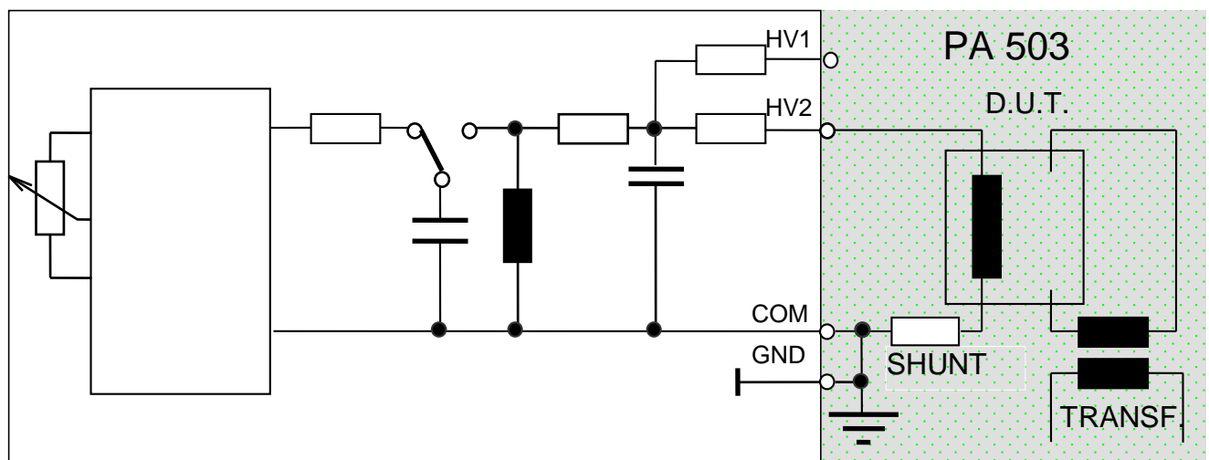
Figure 2: Ring-Wave Generators IPG 612T, schematic, +Safety test cover PA 503, incl. modification of IPG 612T for testing RCCB's acc. to IEC 1008-1.
